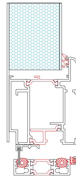
Threshold Detail
